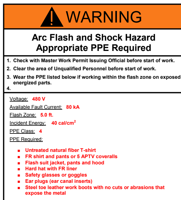
Figure 9-54 Example Arc Flash Warning Label (United States)
