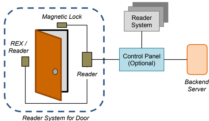
Figure 12-4 Example of an Access Control System Topology
